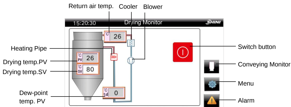
Picture 4-3: Drying Monitoring Screen
