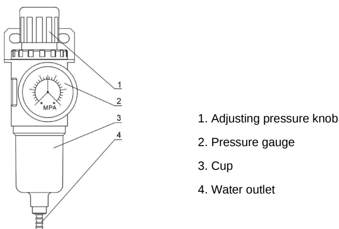
Picture 6-1: Filter & Pressure Regulating Valve Drawing
