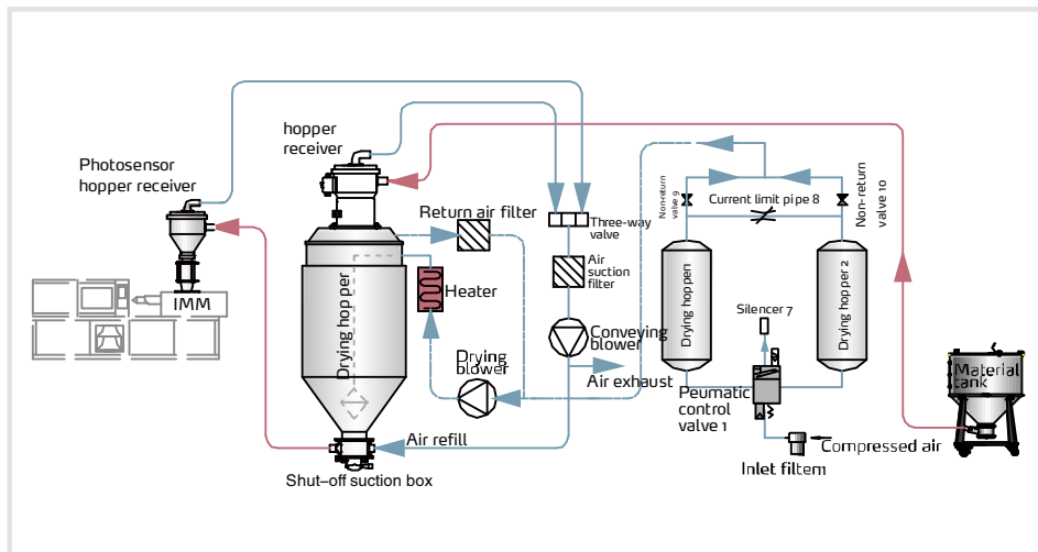
Picture 2-2: SDL-U-HD Working Principle
