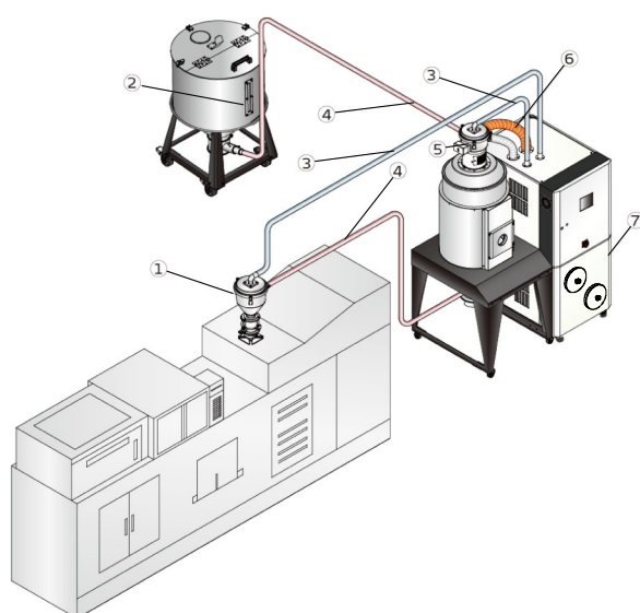
Picture 3-1: Installation Diagram
