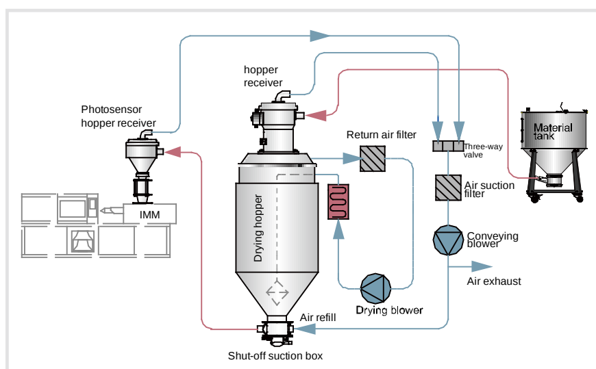
Picture 2-1: SDL-U Working Principle
