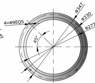
SHR-36U-ST-SHR-48U-ST Base Flange
