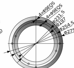
SHR-6U-S-SHR-24U-S Base Flange
