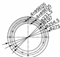
SLHR-6U-24U-S mounting base
