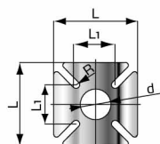
SLHR-U-ES mounting base
