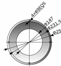
SHR-3U-S Base Flange
