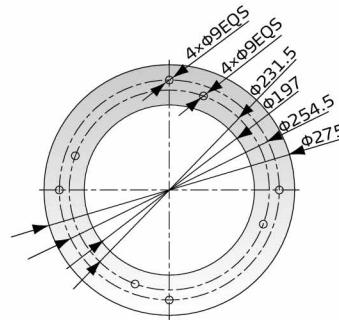
Mounting Base
