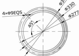
SLHR-36U-96U-S mounting base
