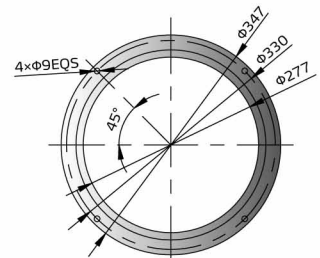
SHR-36U-S-SHR-96U-S Base Flange
