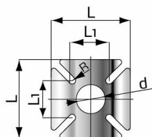
SHR-U-EST Base Flange
