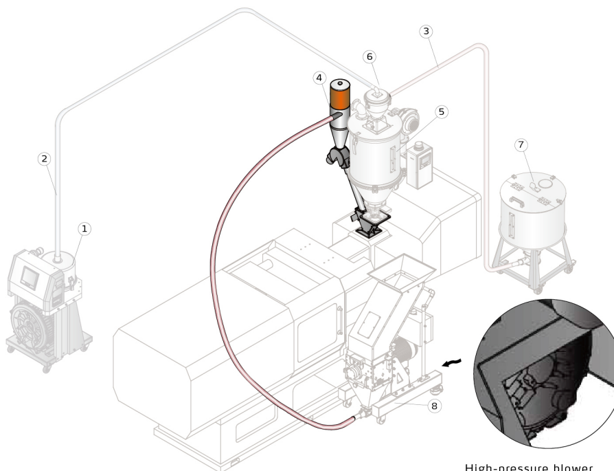
High-pressure blower
