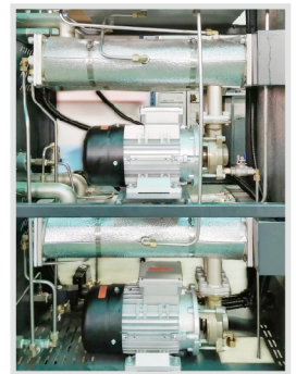
Inner structure
