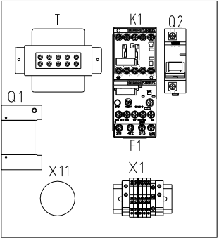
电控箱底板 Base plate of control box
