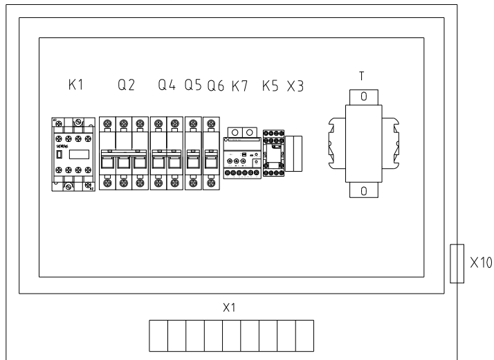
X10 (Heavy-Duty Connector 10P) X10(重载接头10P)
