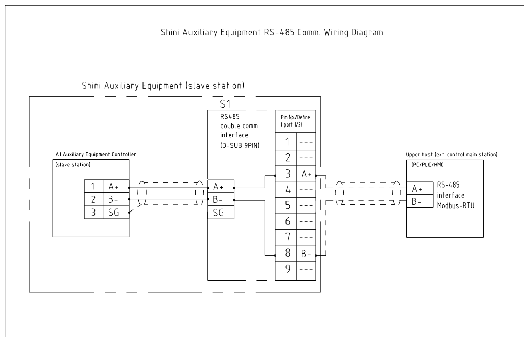
Shini RS-485 Interface Define
