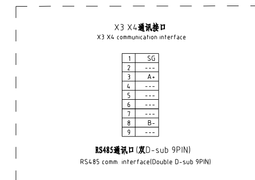
RS485通讯接线图 RS485 Comm. wiring diagram
