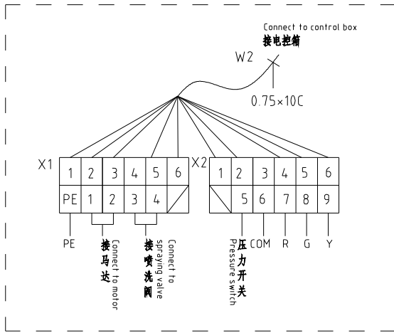
端子排接线图 Terminal block wiring diagram
