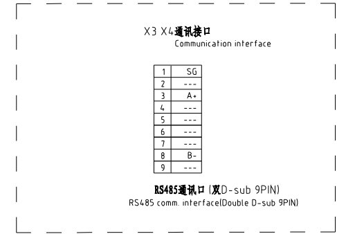
RS485通讯接线图 RS485 Comm. wiring diagram
