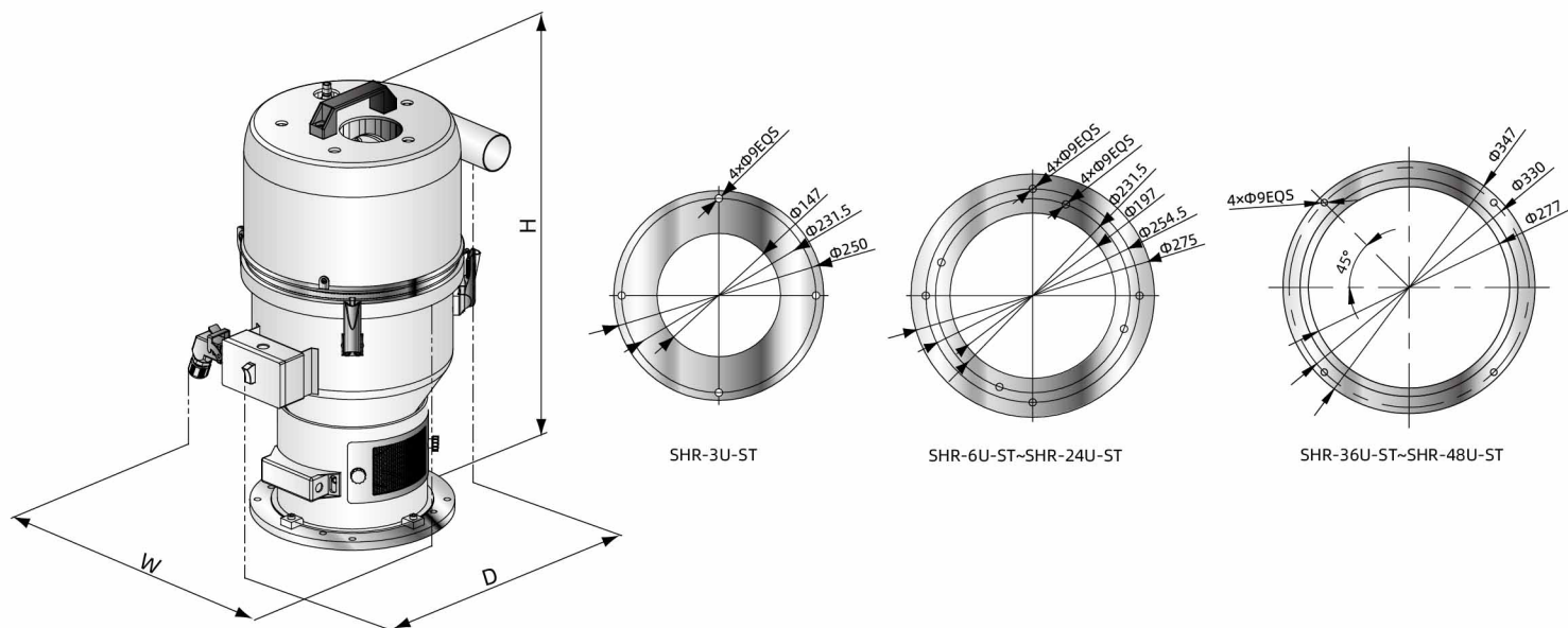
SHR-U-ST规格表
