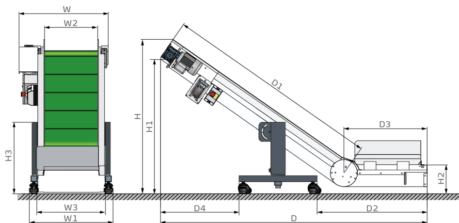
CB Outline Drawing
