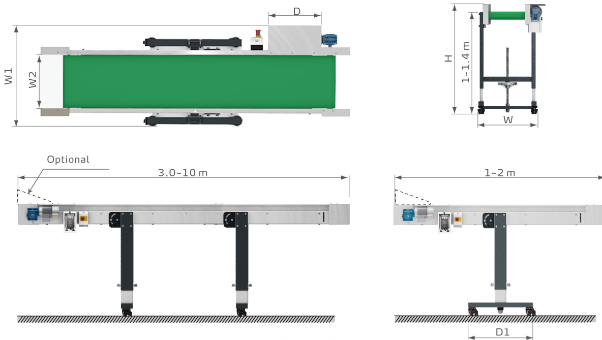
PNL Outline Drawings
