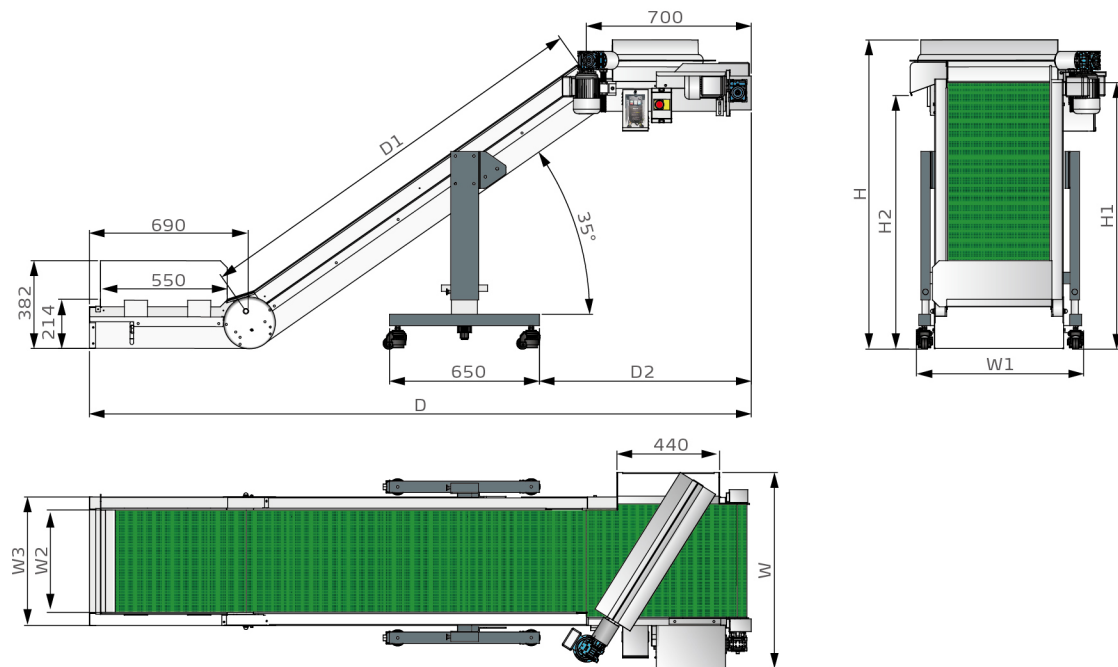
CBD Outline Drawings
