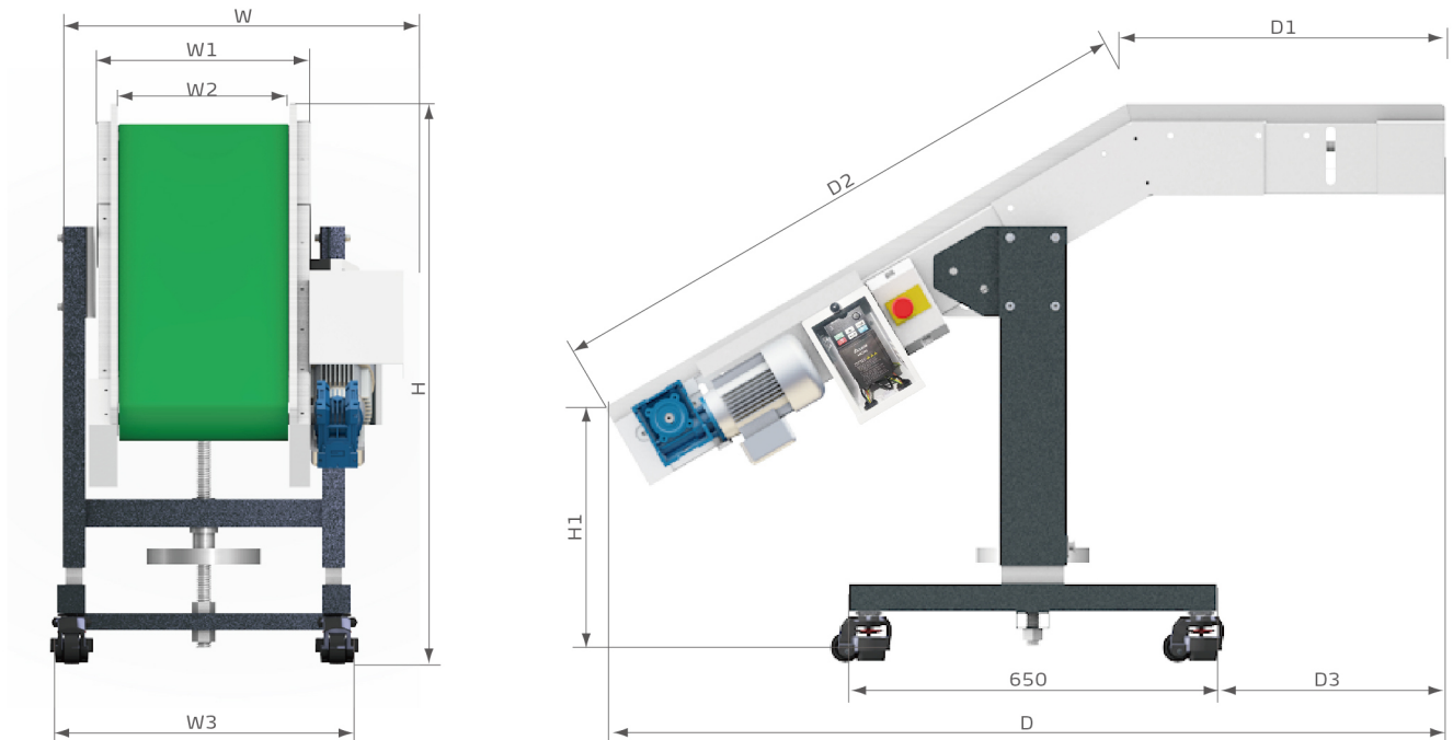
SV Outline Drawings
