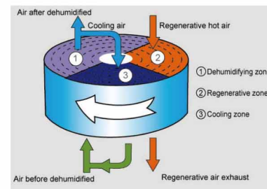
Honeycomb Rotor Working Principle
